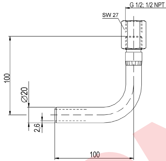
Elbow 90°
